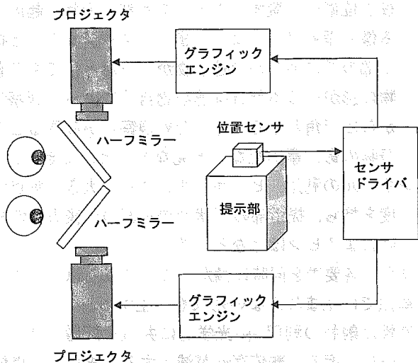
図6 MEDIA X'talの構成図 Fig.6 System architecture of MEDIA X'tal.
